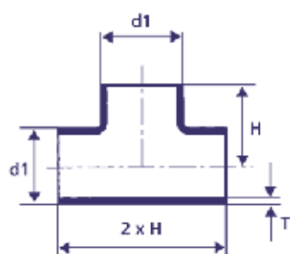
EQUAL TEES WITH BRANCH
