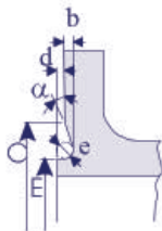
Type H 'O' Ring Groove
